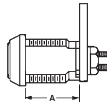
Lock Length
